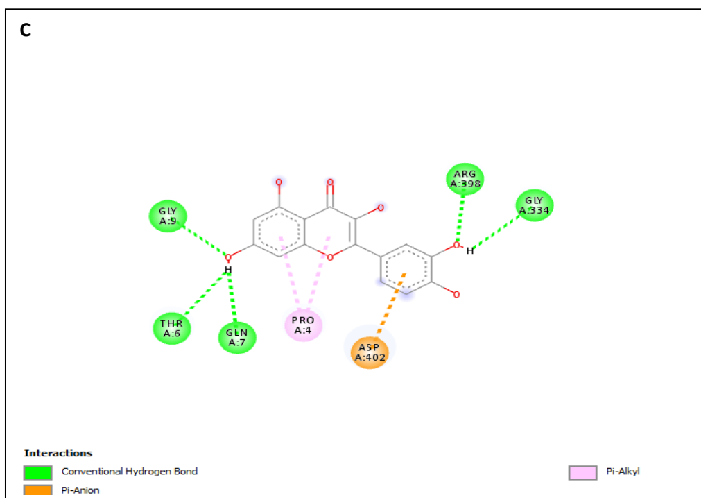
Fig. 3. Molecular docking of a receptor \alpha -glucosidase and the identified ligands, (A) 2D structural interaction of \alpha -glucosidase with catechin, (B) 2D structural interaction of \alpha -glucosidase with conduritol A, (C) 2D structural interaction of \alpha -glucosidase with Quercetin
