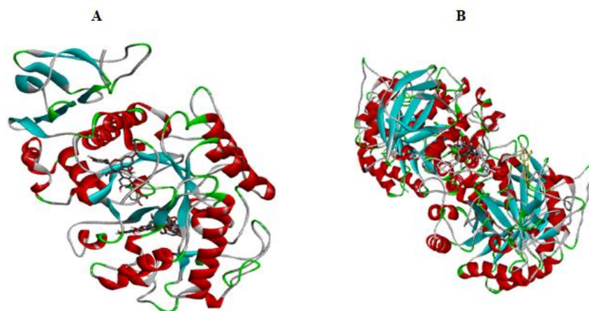
Fig. 1. (A) The crystal structure of \alpha -Amylase, (B) The crystal structure of \alpha -Glucosidase
