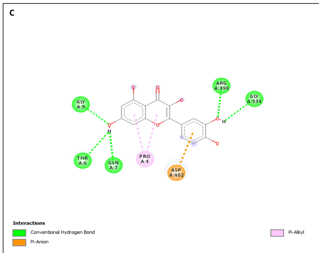
Fig. 2. Molecular docking of a receptor \alpha -amylase and the identified ligands, (A) 2D structural interaction of \alpha -amylase with catechin, (B) 2D structural interaction of \alpha -amylase with conduritol A, (C) 2D structural interaction of \alpha -amylase with Quercetin
