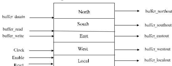
Fig.10. Schematic of Buffer
