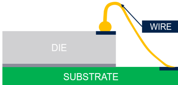
Fig. 1. Wire Bonding Connection
