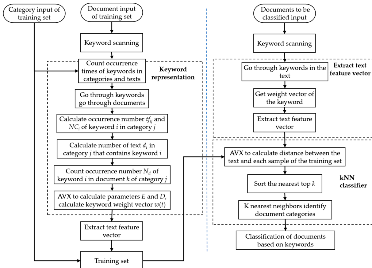
Figure 2. The procedure of text classification algorithm with AVX-256 acceleration.
