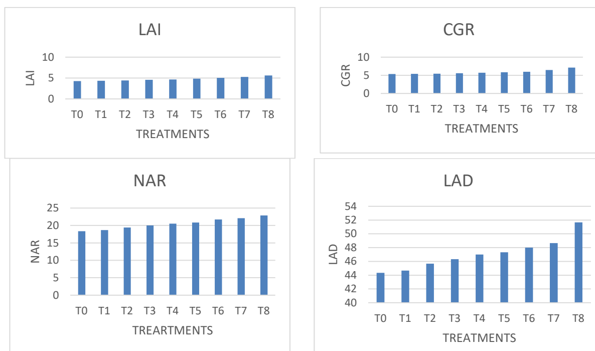
Fig. 2. Average data of growth parameters leaf area index, leaf area duration (days), crop growth rate ( \text{gm}^{-2}\text{day}^{-1} ), net assimilation rate ( \text{gm}^{-2}\text{day}^{-1} )
