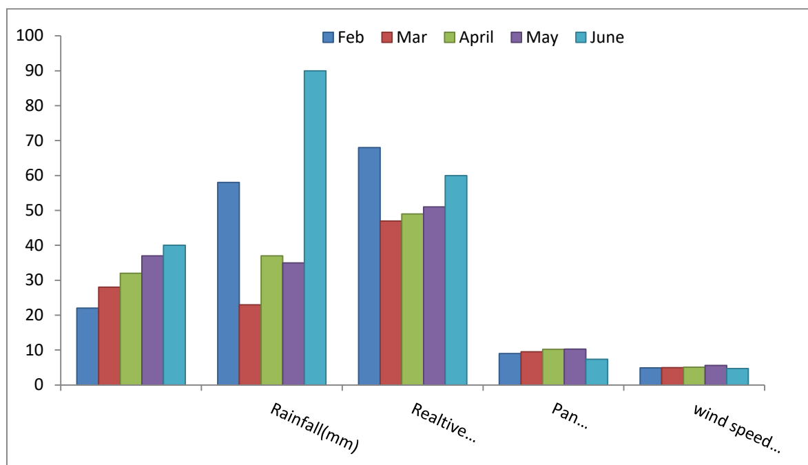
Fig. 1. Average monthly data of temperature (°C), Rainfall (mm), relative humidity (%), Pan evaporation (mm) and wind speed (km/h)
