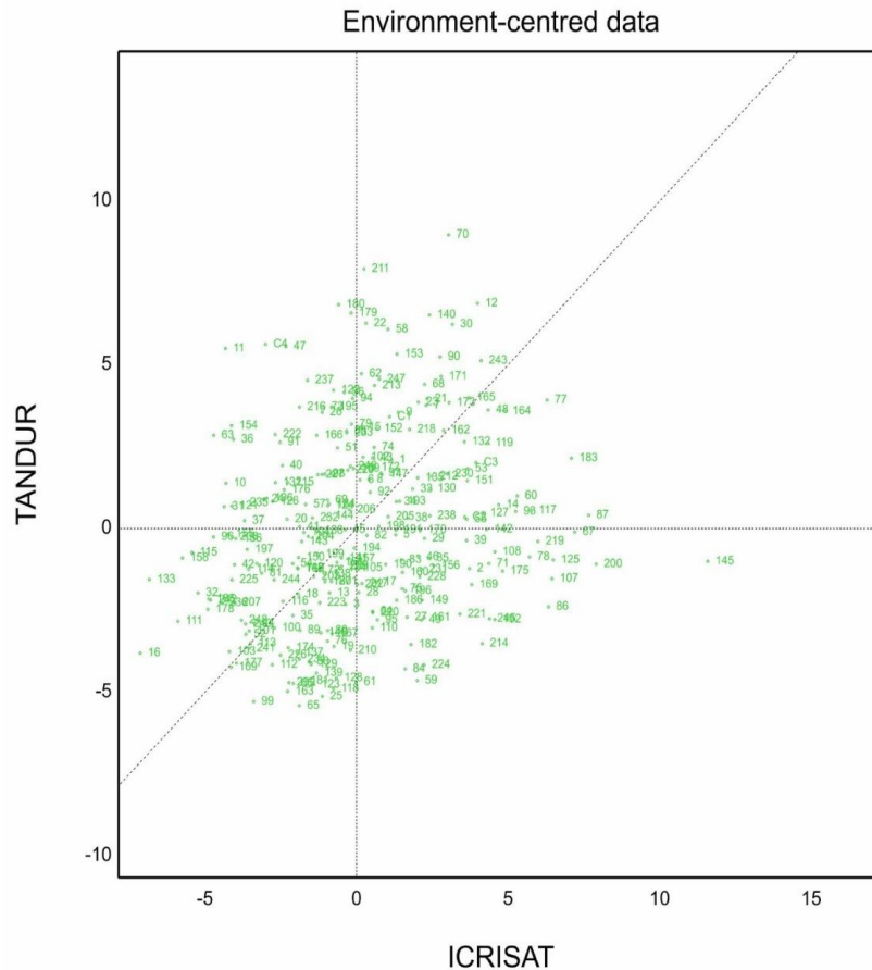
Fig. 1. Centered scatter plot for seed yield at ICRISAT, Patancheru and ARS, Tandur
