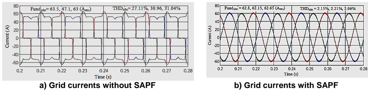
Fig. 16. Grid currents before and after application of SAPF
