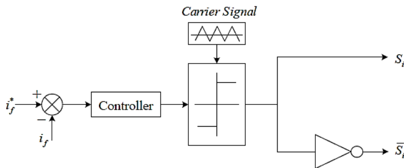
Fig. 5. The Sinusoidal PWM Control Method for the VSI [14]
