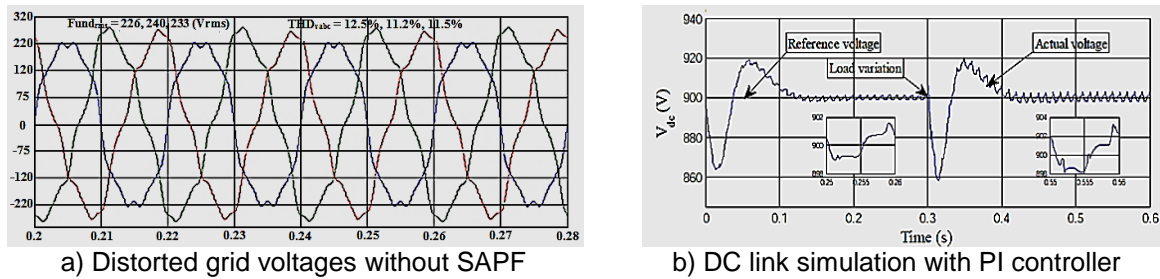
Fig. 14. Distorted grid voltages without SAPF and dc link simulation with PI controller
