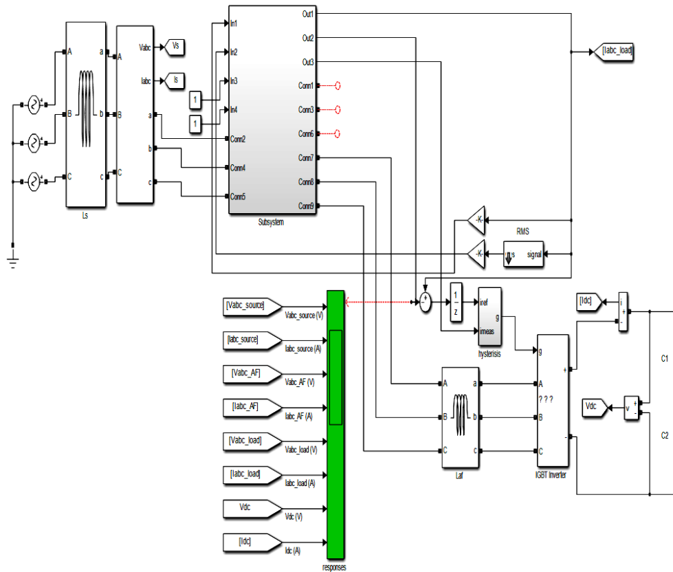
Fig. 8. Voltage Source Inverter showing the 3-Phase Source
