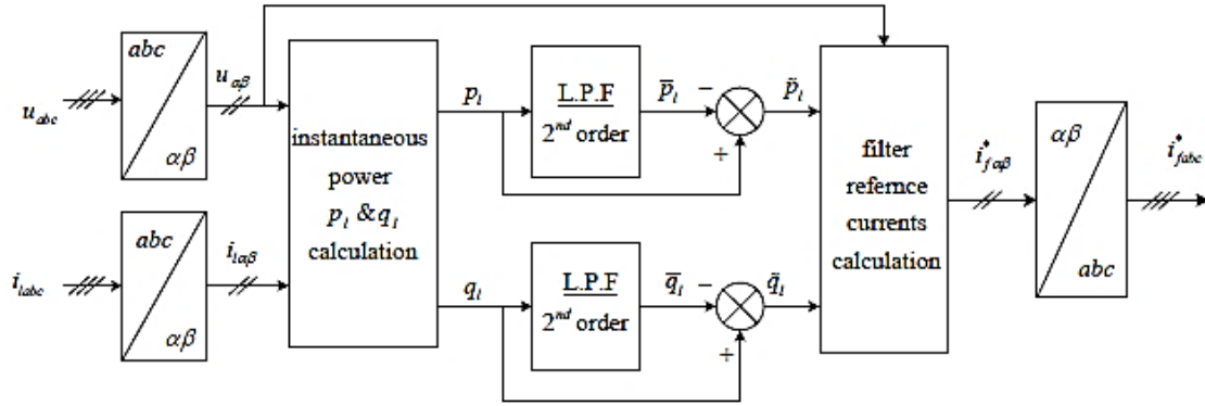
Fig. 2. Principle of Instantaneous Active and Reactive Power Theory [14]
