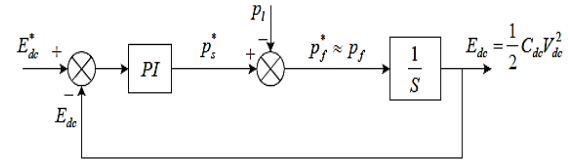
Fig. 7. DC Voltage Closed Loop Control
