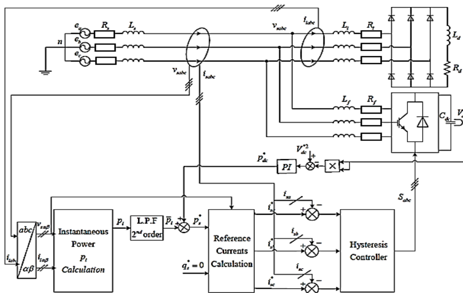
Fig. 6. Indirect control of SAPF based on the instantaneous power theory [14]
