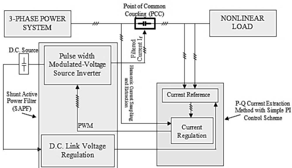
Fig. 1. Block Diagram of the Shunt Active Power Filter
