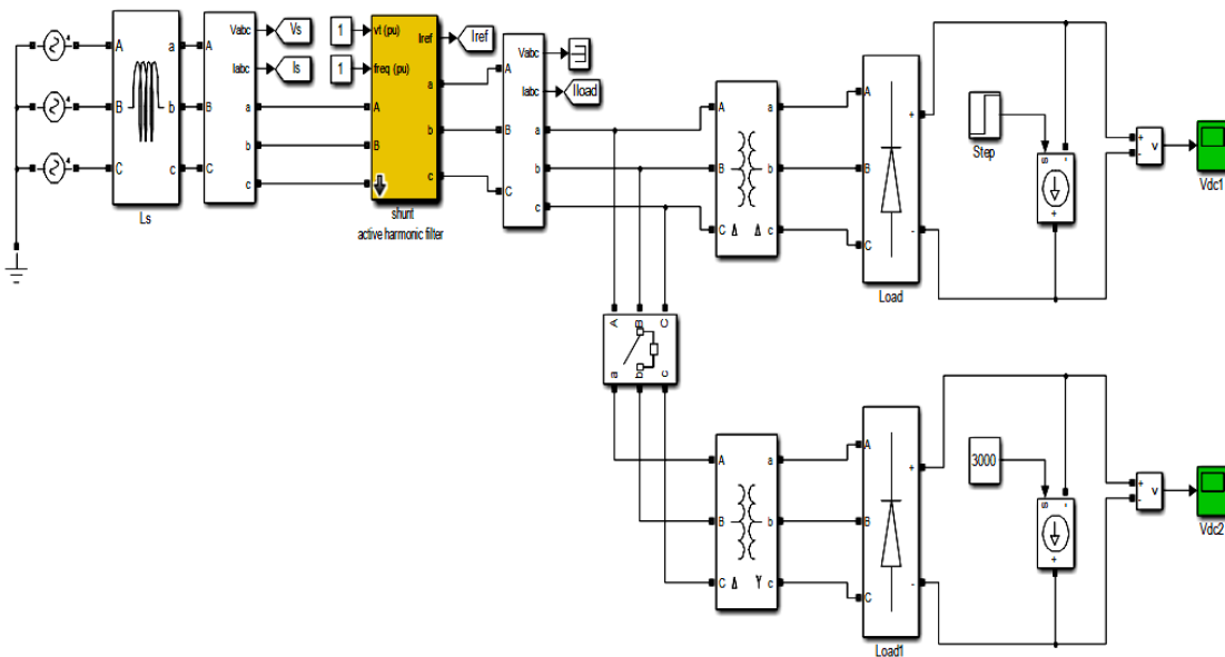
Fig. 13. Second Simulation output with different loads with the SAPF connected
