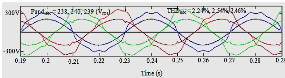
Fig. 15. Filtered unbalanced system voltages after application of SAPF
