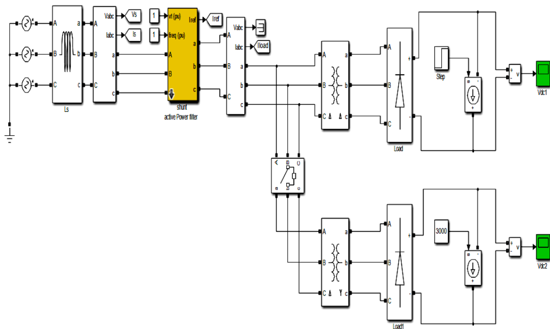
Fig. 11. Complete model of the system
