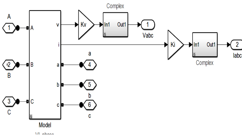
Fig. 9. The PI Controller for the Reference Current generation and Control
