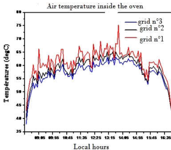
Fig. 5. Air temperatures through the racks
