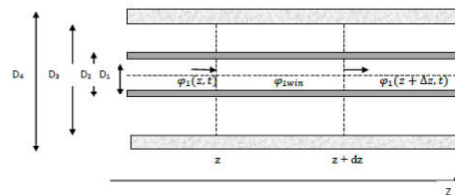
Fig. 3. Longitudinal section of heat transfer tube
