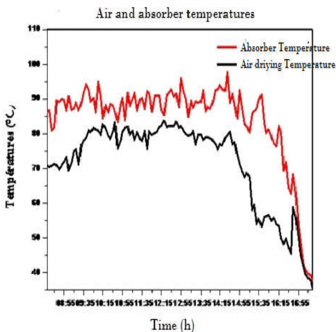
Fig. 6. Temperature development of the absorber and drying air
