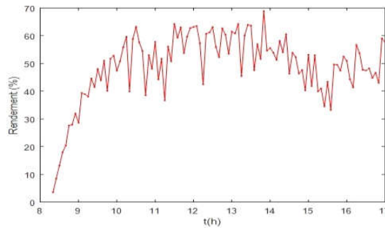
Fig. 7. Development of the thermal efficiency of the concentrator
