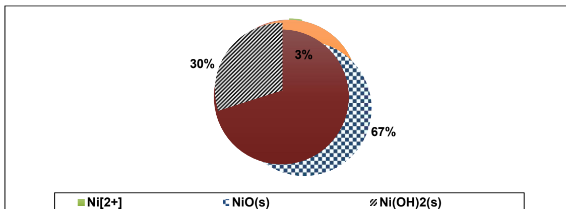
Fig. 10. Proportional plot of Ni species in surface water of Woji creek
