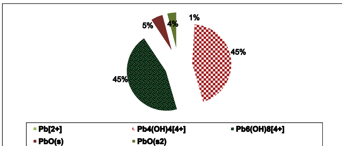
Fig. 7. Proportional plot of Pb species in surface water of Woji creek
