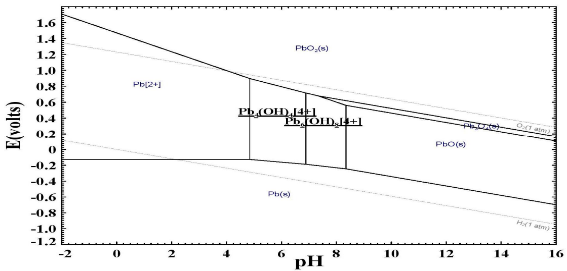
Fig. 6. Pourbaix diagram for Pb in the surface water
