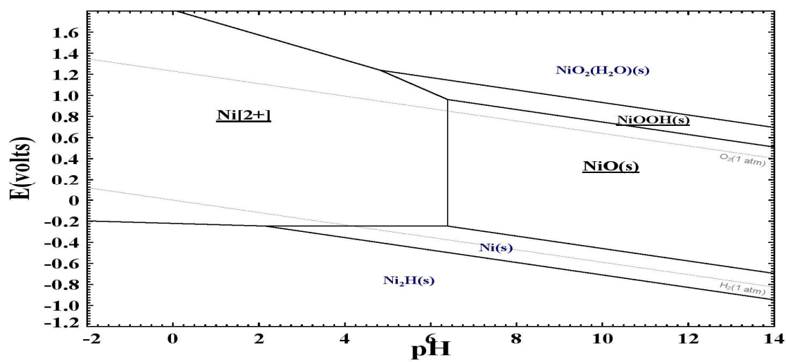
Fig. 9. Pourbaix diagram for Ni in the surface water
